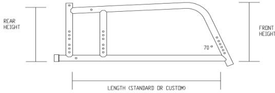
Frame Dimensions
